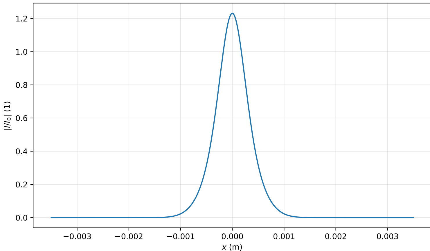
Intensity profile I(x, y = 0, z = 0.796m)/I_0 , P_{in}=0.8P_{cr} , artificial time
